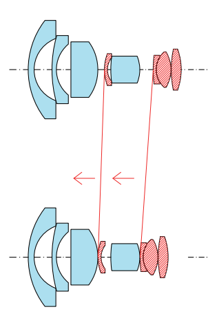
Floating Lens
