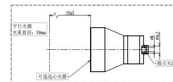
NTD33IR055W220M42-I
