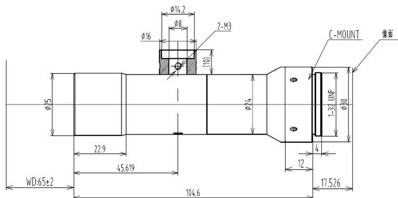
MT231R4W65C-L
