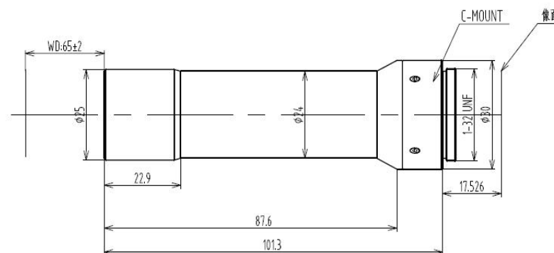
MT231R4W65C-I
