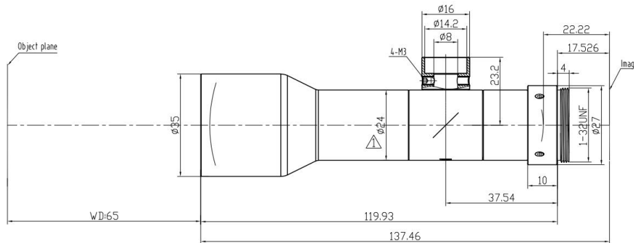
MT23IR05W65C-L
