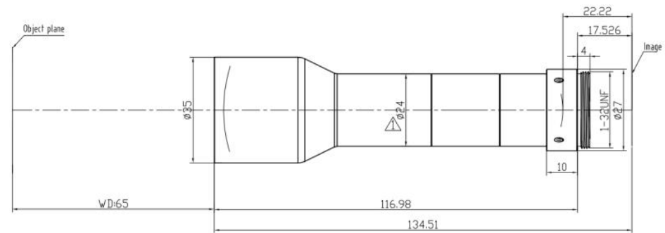
MT23IR05W65C-I
