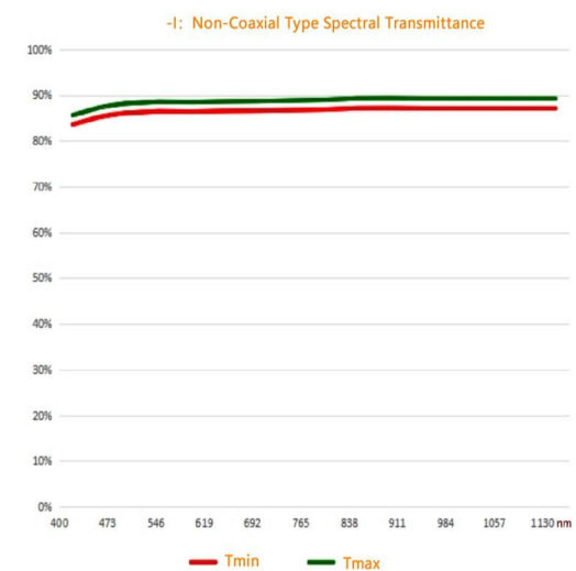
MT23IR05W65C-I
