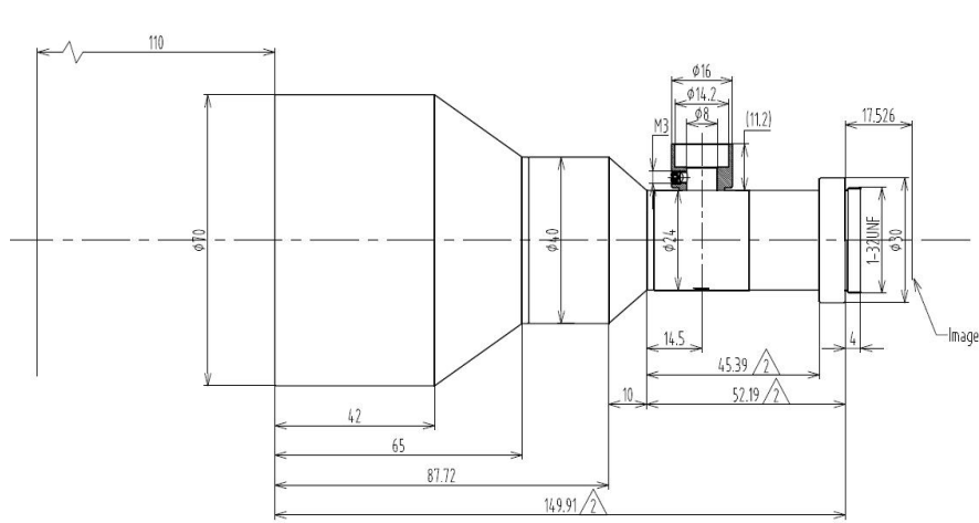
MT23IR03W110C-L
