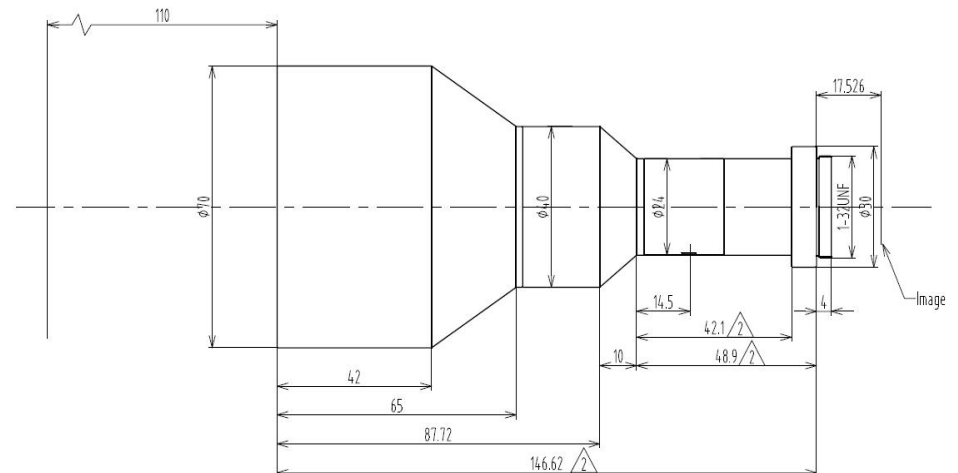
MT23IR03W110C-I
